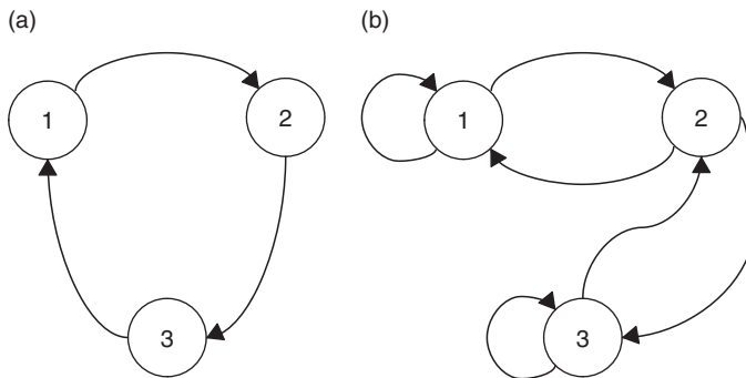
Figure 4. Transition graphs of two Markov chains with (a) only one periodic orbit and (b) an invariant, ergodic and mixing equilibrium state.
